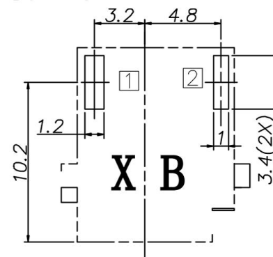
P. C. B Layout (Printed-side view)
