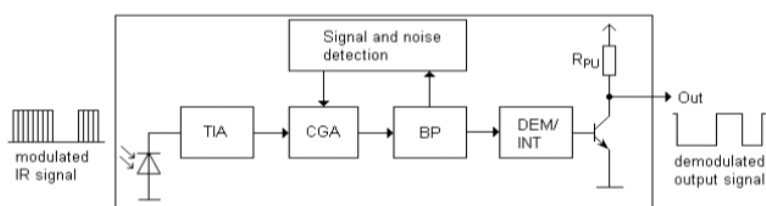
Fig.1 Block Diagram
