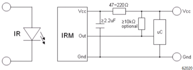
Fig.9: application circuit
