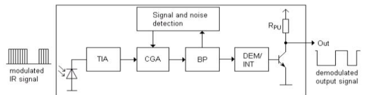
Fig.1 Block Diagram
