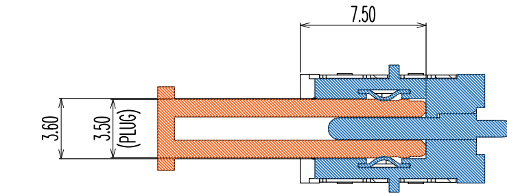
MATING PLUG SECTION
