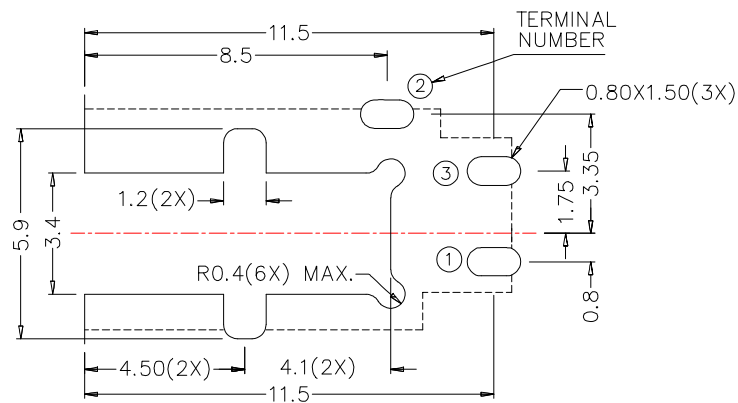
P.C.B LAYOUT MOUNTING PATTERN (TOP VIEW)
