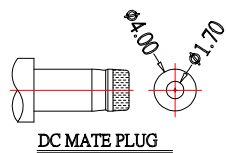
DC MATE PLUG
