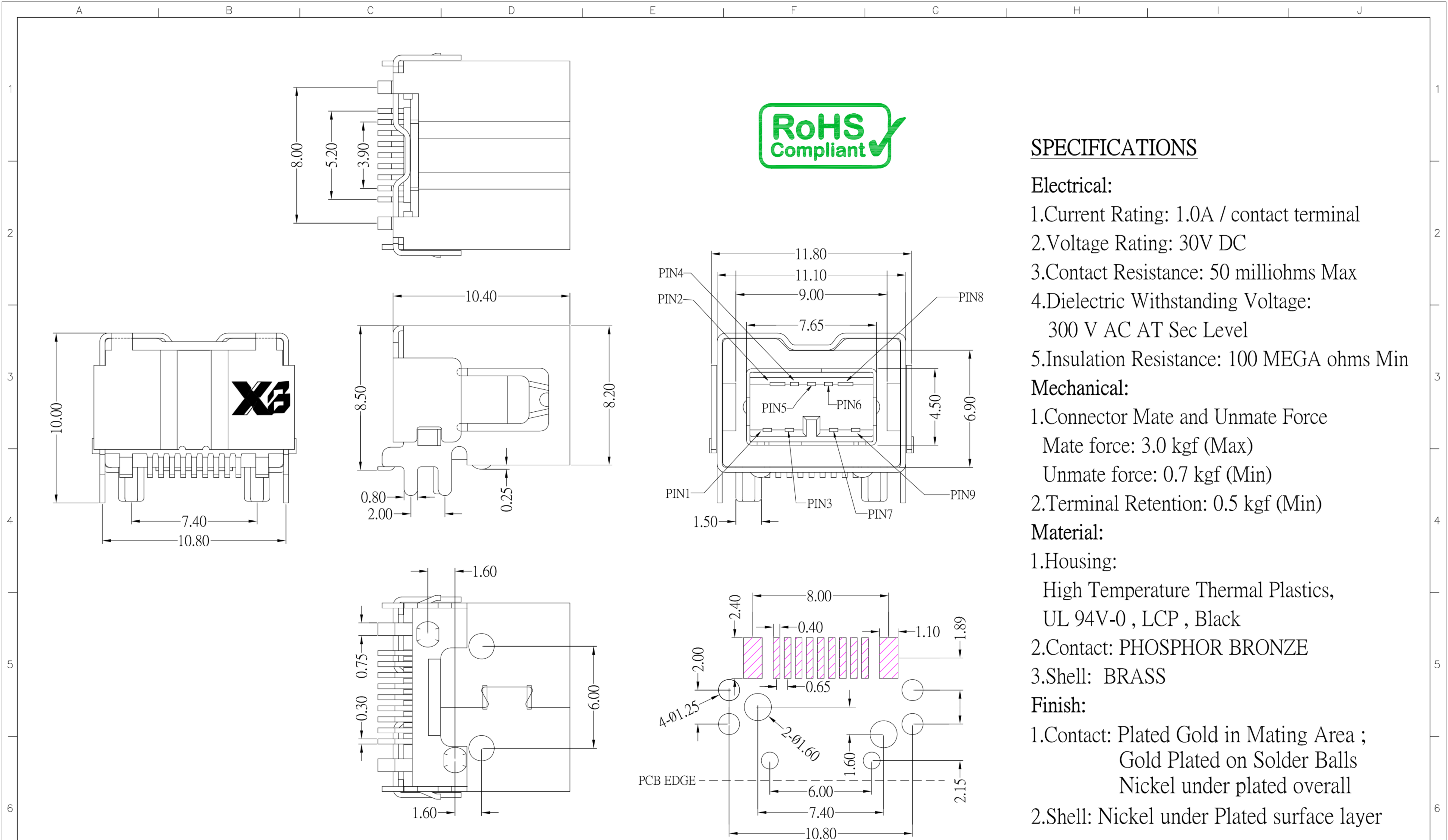
P.C.B LAYOUT MOUNTING PATTERN
