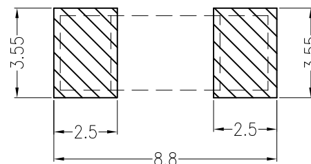
Board Layout
