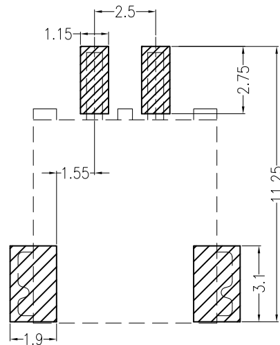
Board Layout
