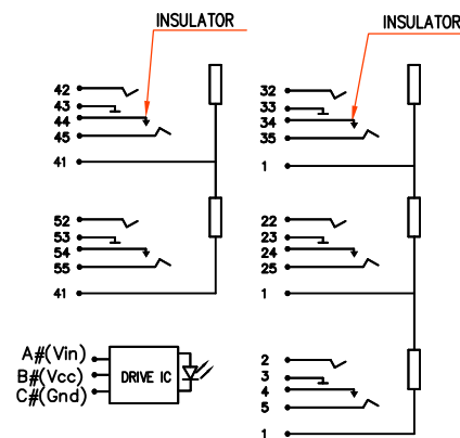
CIRCUIT SCHEMATIC
