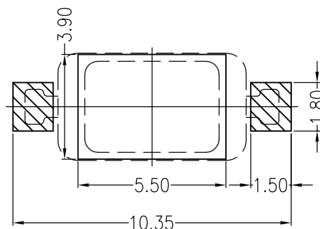
Board Layout
