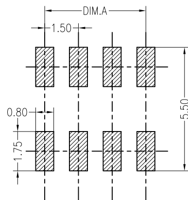
Board Layout
