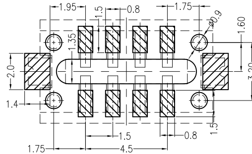
Board Layout
