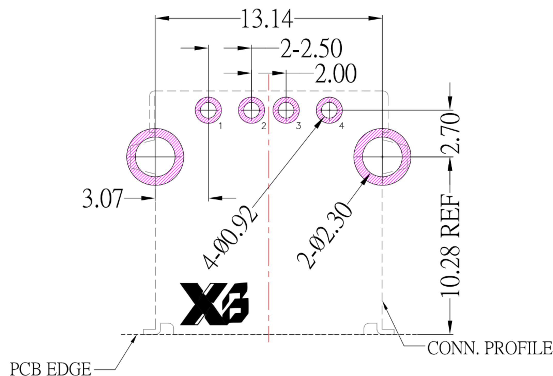
P.C.B LAYOUT MOUNTING PATTERN(TOP VIEW)
