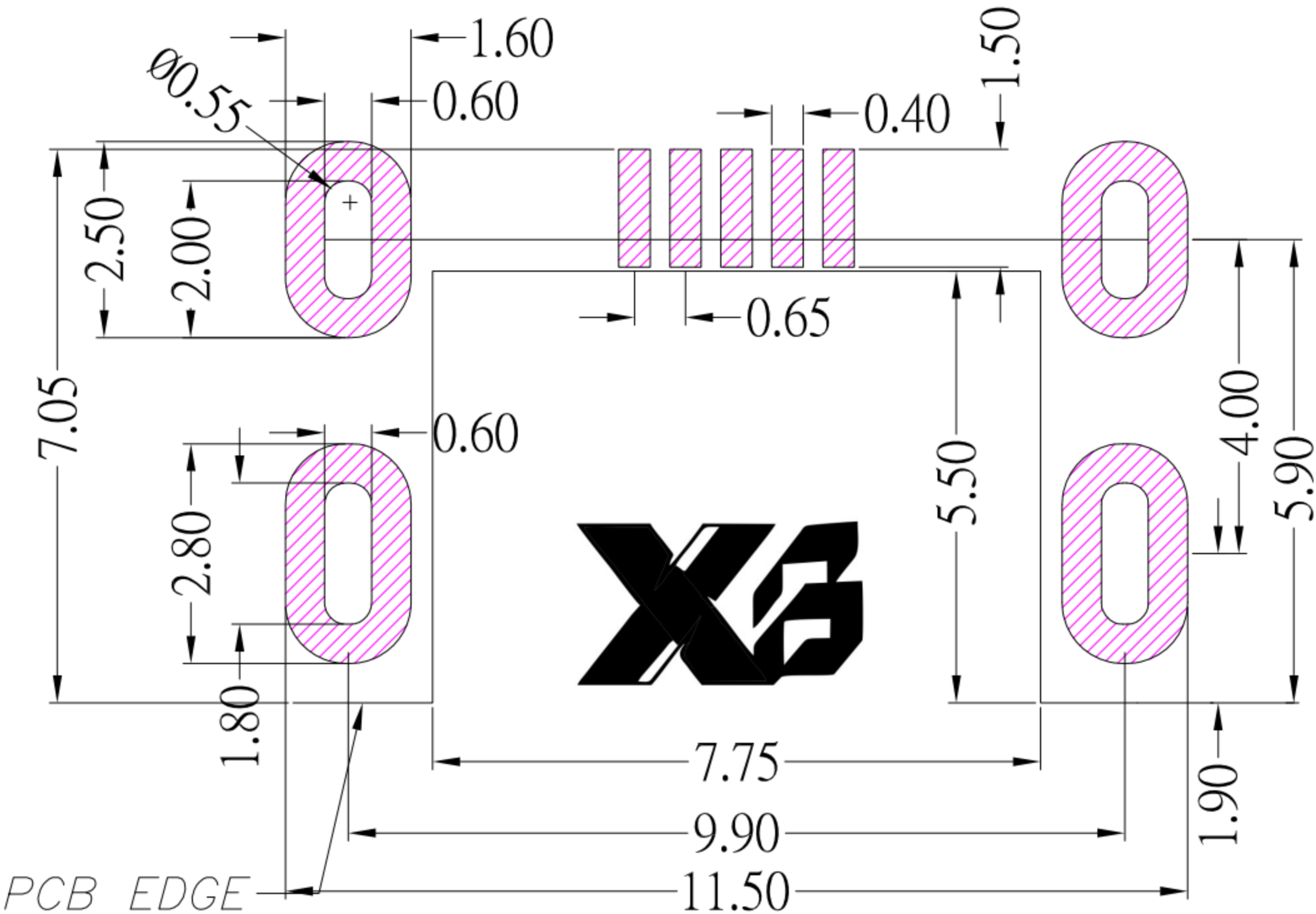
P.C.B LAYOUT MOUNTING PATTERN
