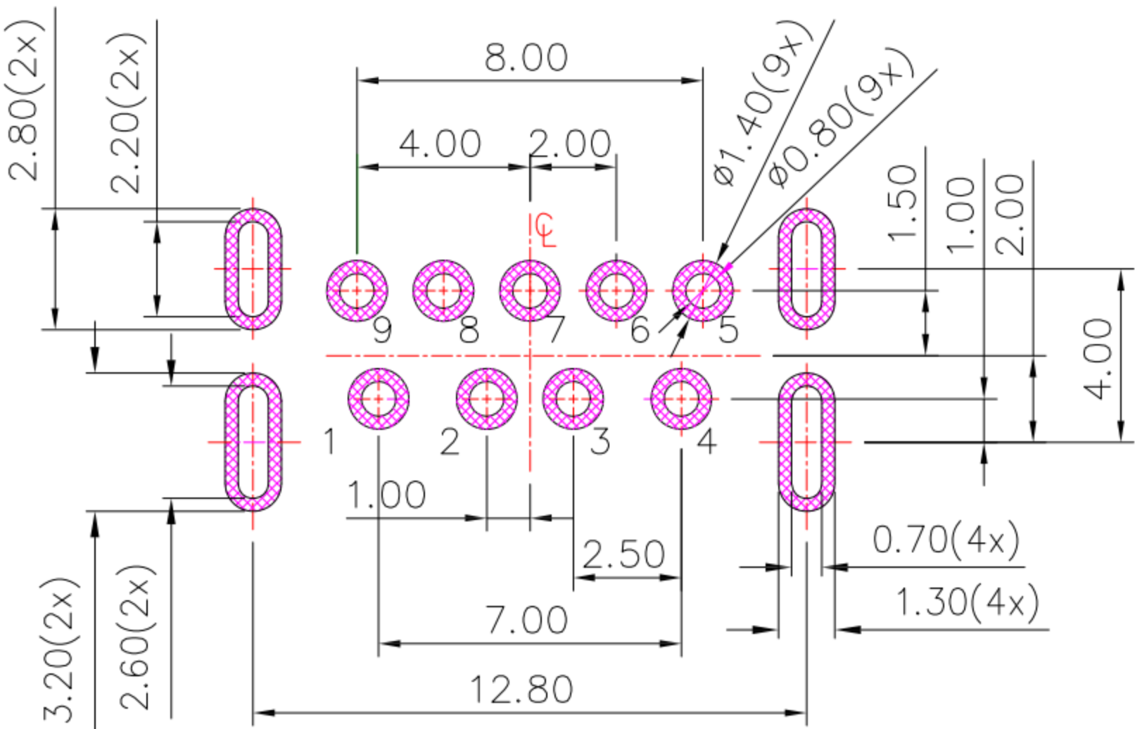
P.C.B LAYOUT MOUNTING PATTERN
