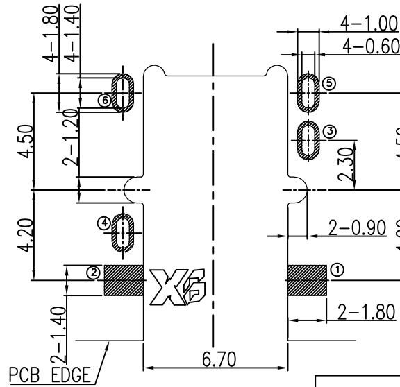
RECOMMENDED PCB LAYOUT(TOP VIEW) (GENERAL TOLERANCE:±0.05)
