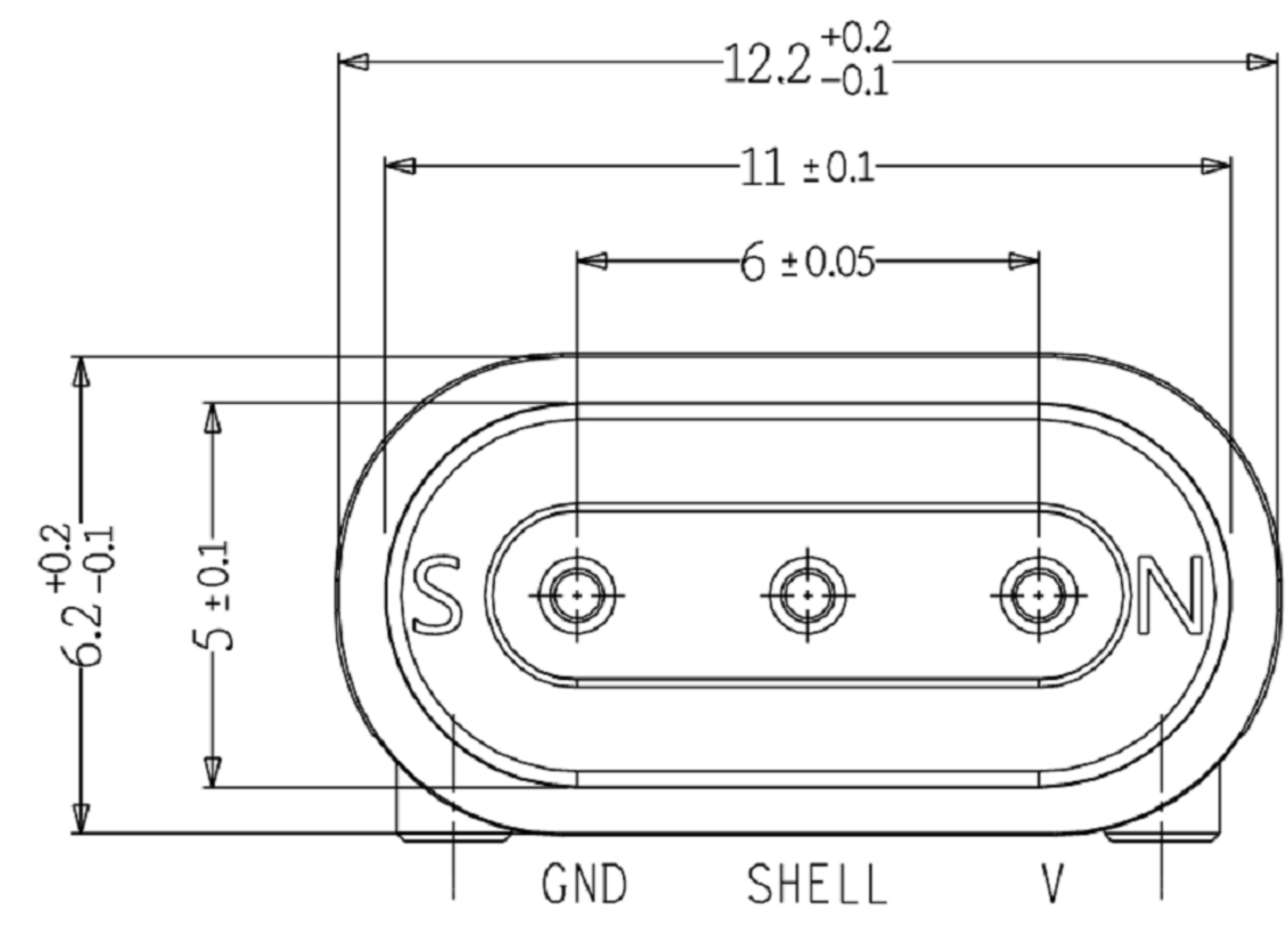
VIEW S SCALE 4/1
