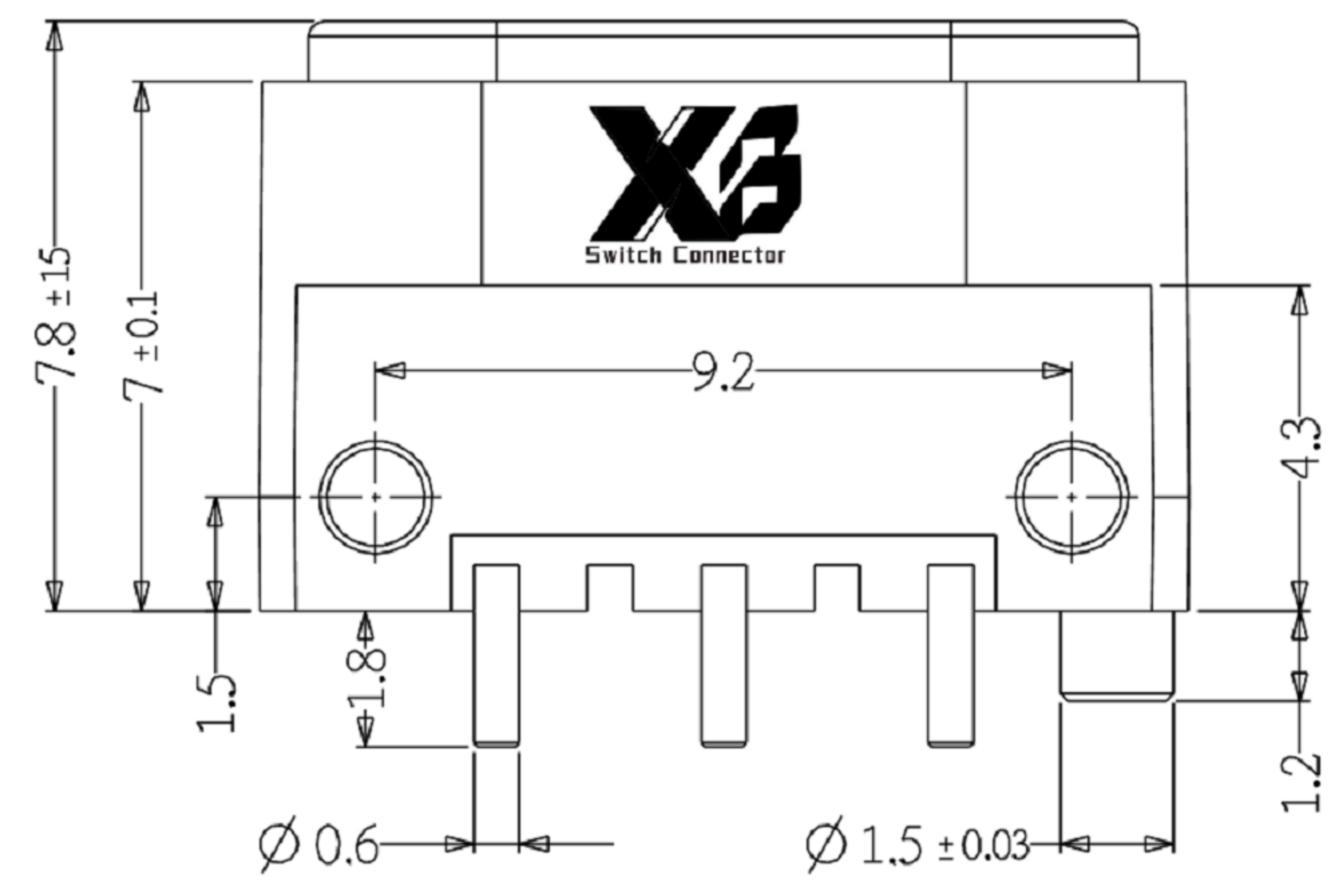
VIEW P SCALE 4/1
