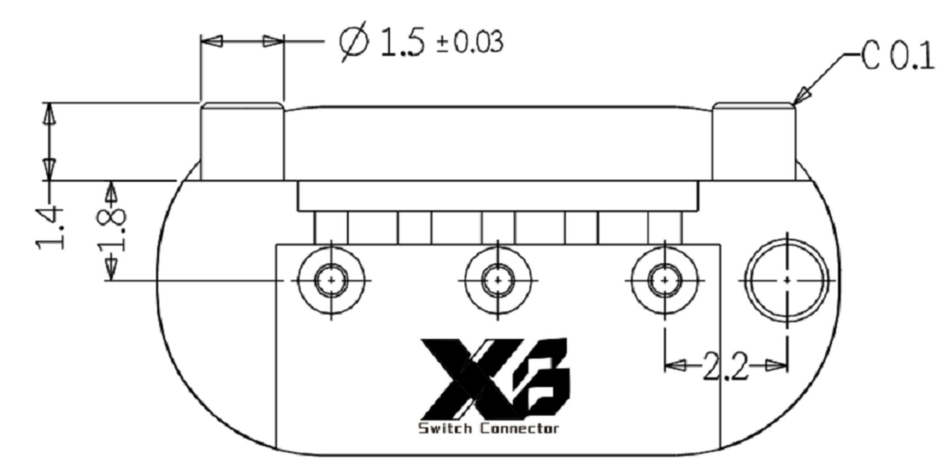
VIEW T SCALE 4/1
