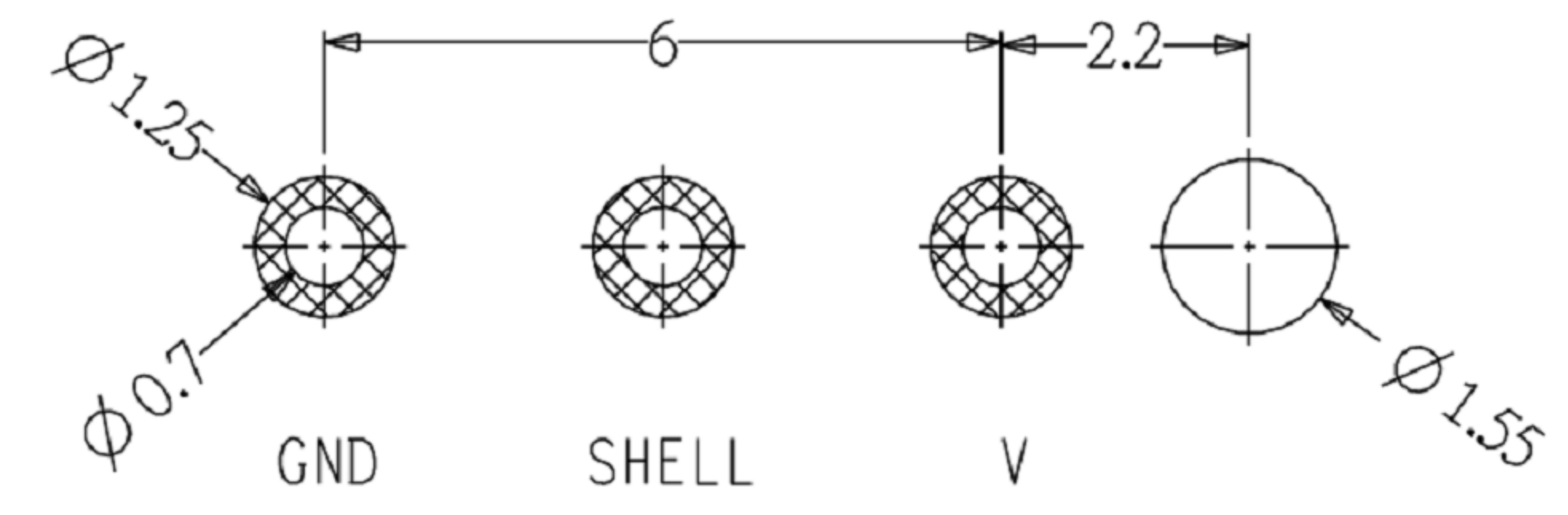
Recommend PCB Layout (TOP VIEW) Layout Tolerance: ±0.05
