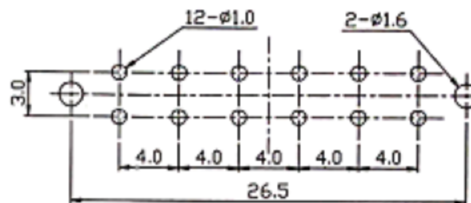
PEIRCING PLAN
