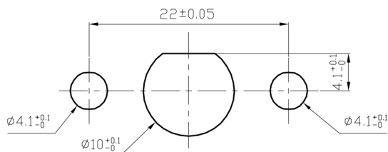
PANEL CUTOUT
