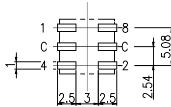
P.C.B DIMENSION (Top View)
