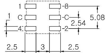
P.C.B DIMENSION (Top View)
