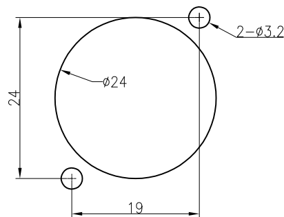
Panel cut out (rear side)
