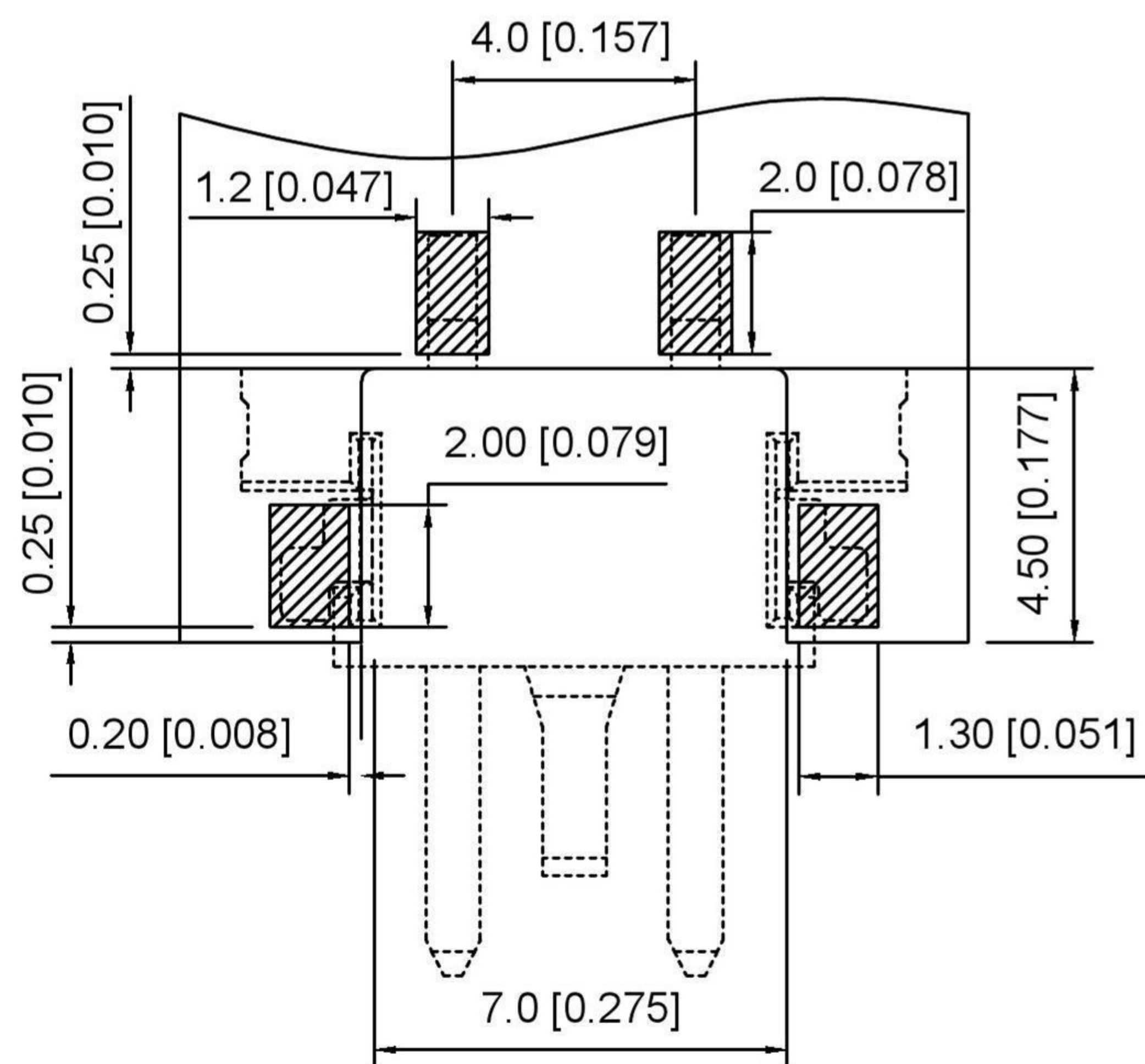
PCB LAYOUT
