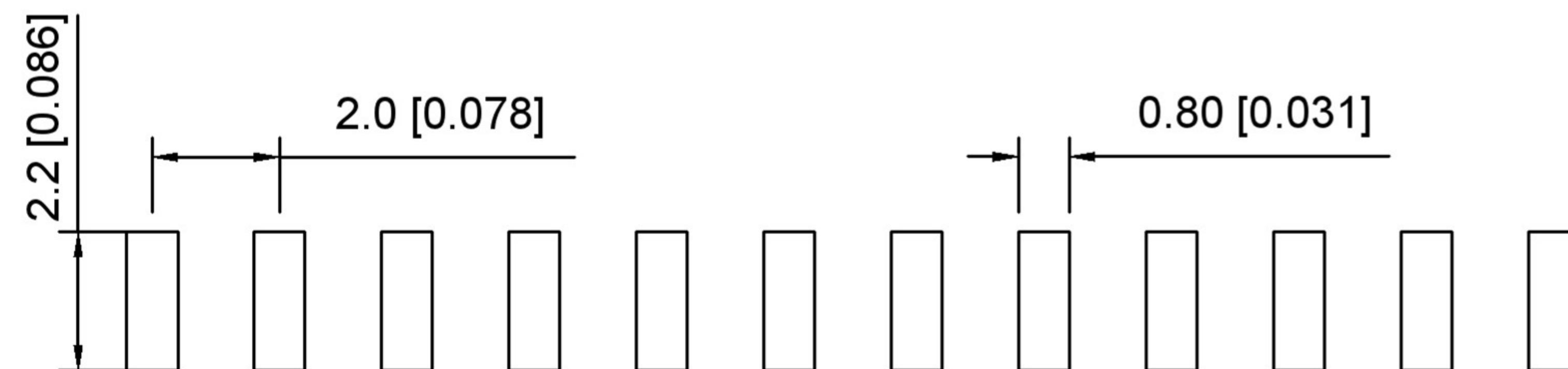
PCB LAYOUT
