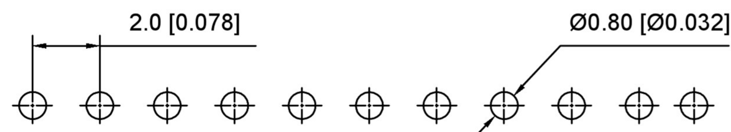
PCB LAYOUT
