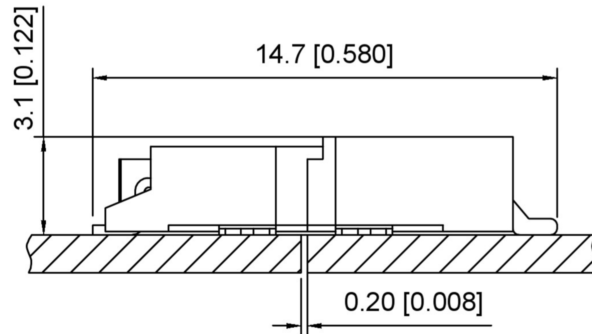
Assembly Layout
