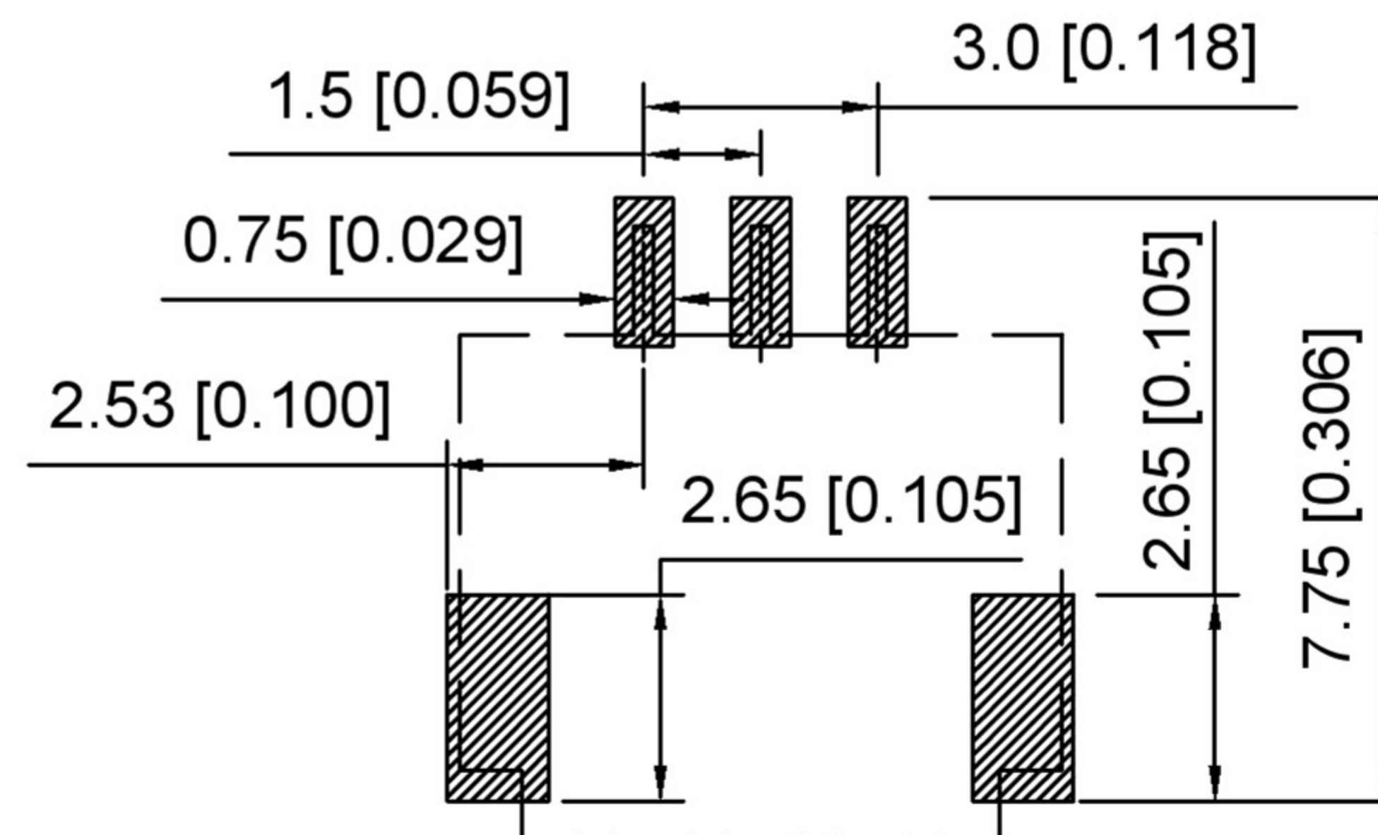
Board Layout General Tolerance:±0.05
