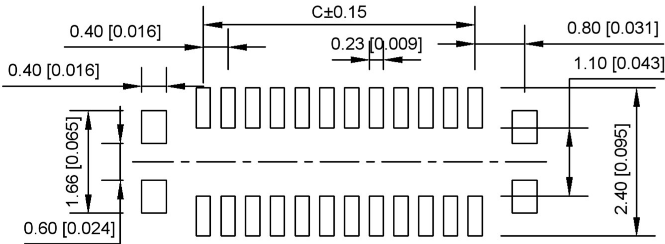
RECOMMENDED PCB LAYOUT CONNECTOR SIDE XB Connecity
