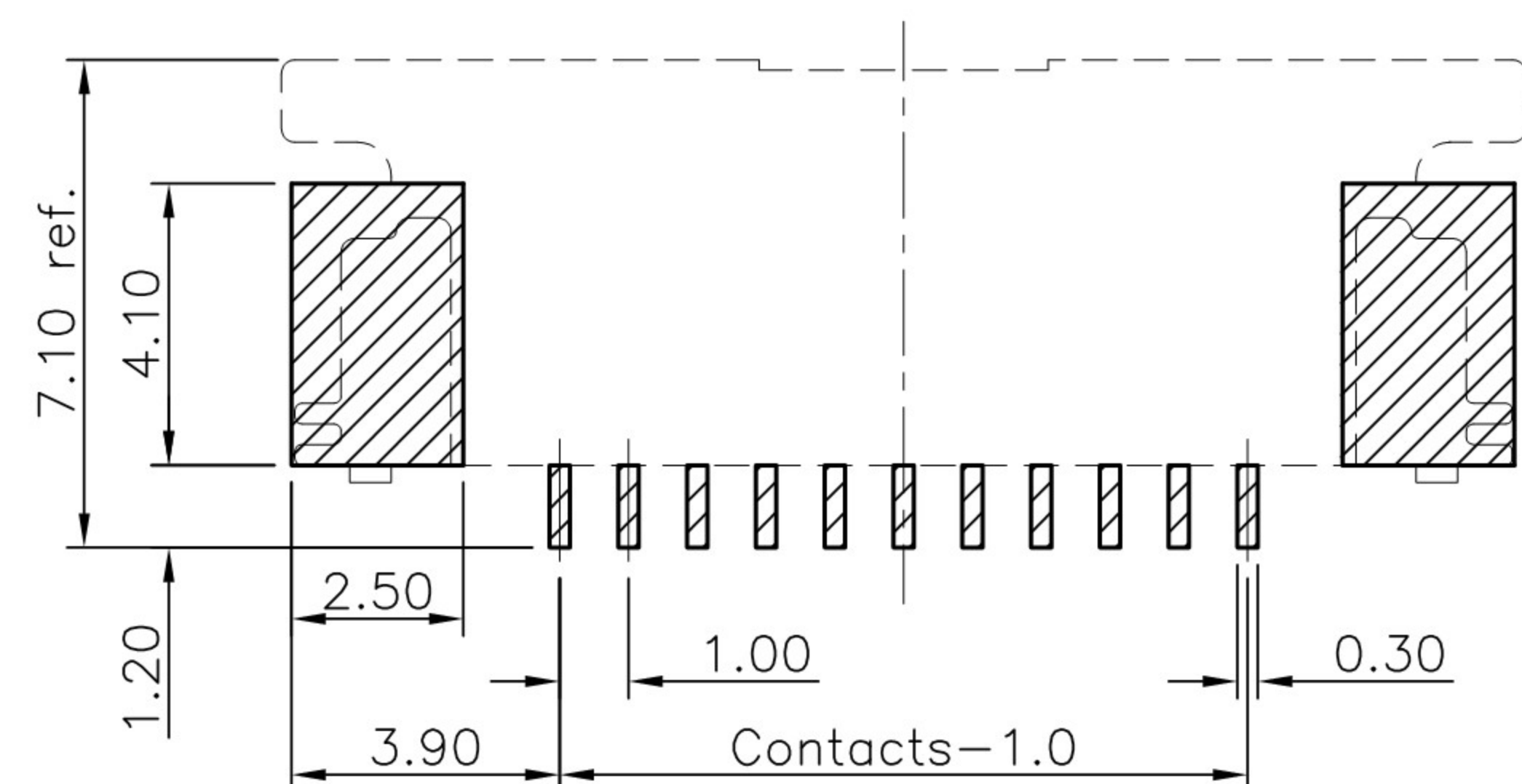
RECOMMENDED LAYOUT (TOP VIEW) GENERAL TOLERANCE: \pm 0.05\text{mm}
