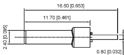
SECT B-B
