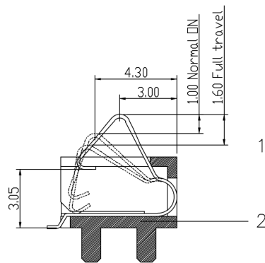
VIEW A-A'
