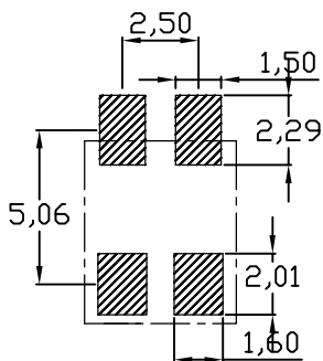
RECOMMENDED PCB LAYOUT TOP VIEW (. XX \pm 0.05)
