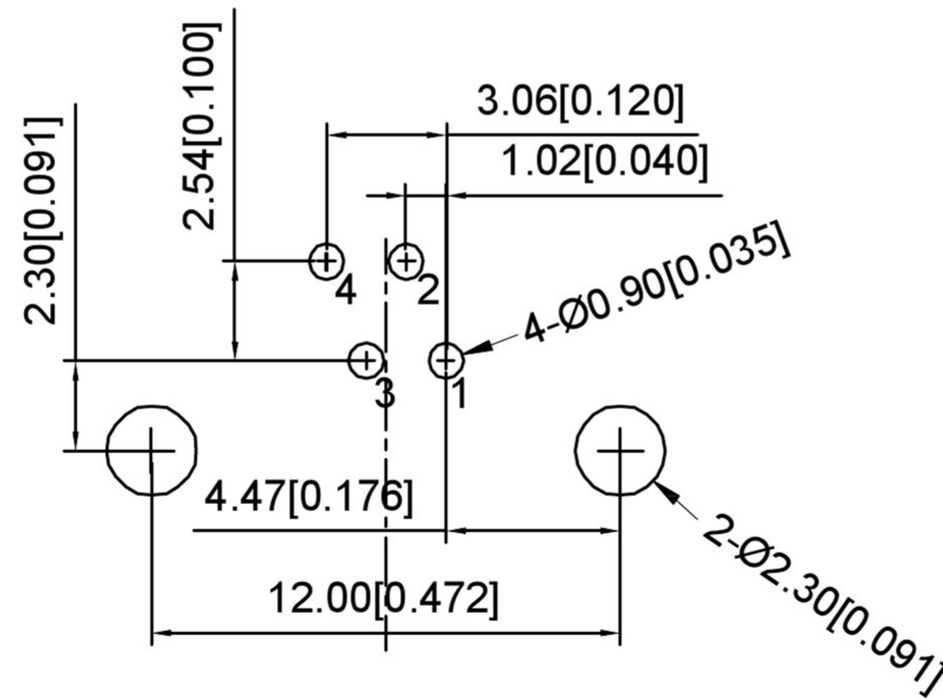
RECOMMENDED PCB LAYOUT VIEWED FROM COMPONENT SIDE
