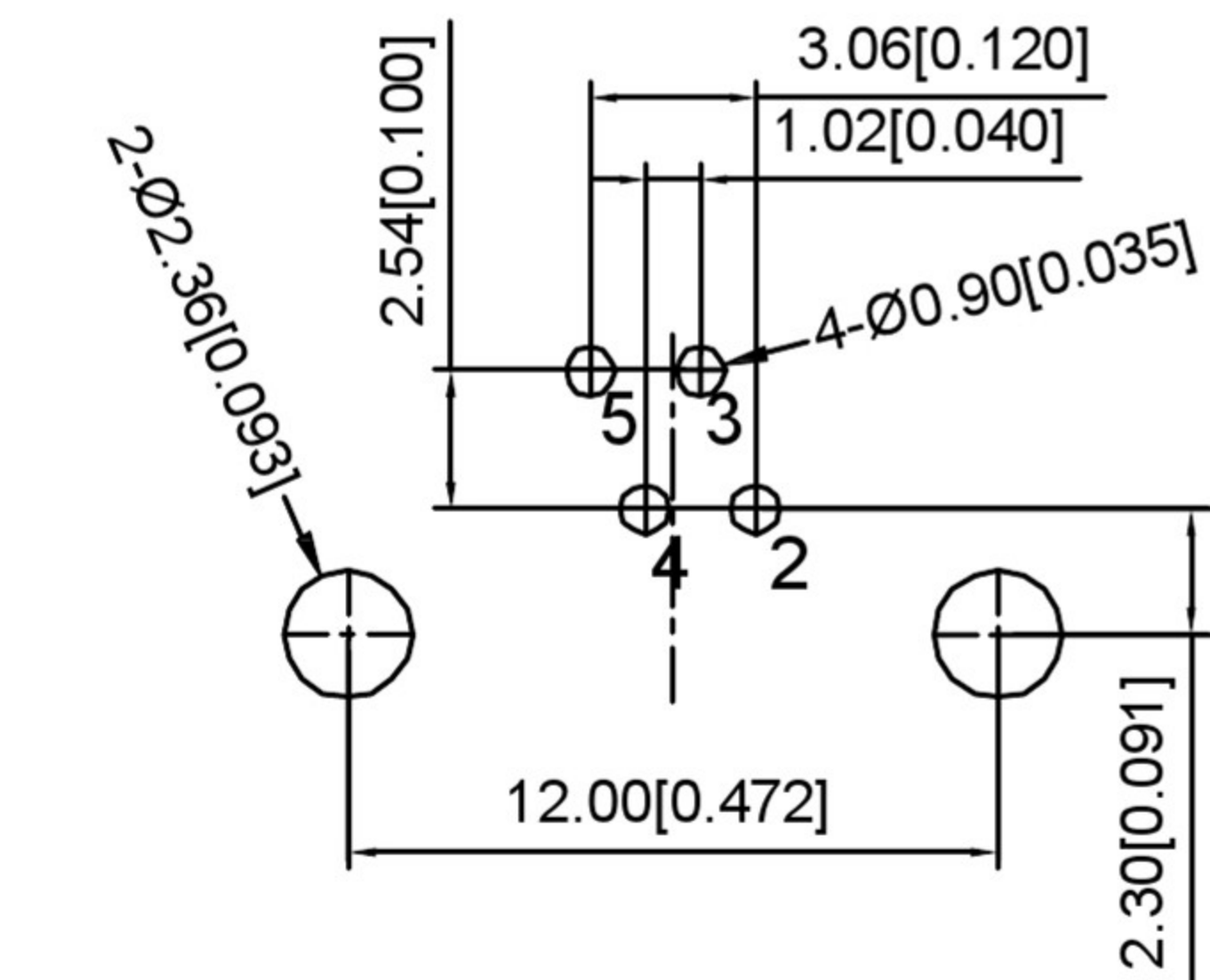
RECOMMENDED PCB LAYOUT VIEWED FROM COMPONENT SIDE
