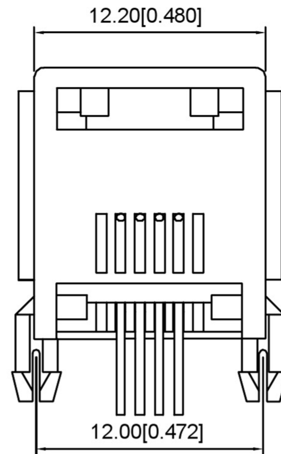
BACK VIEW
