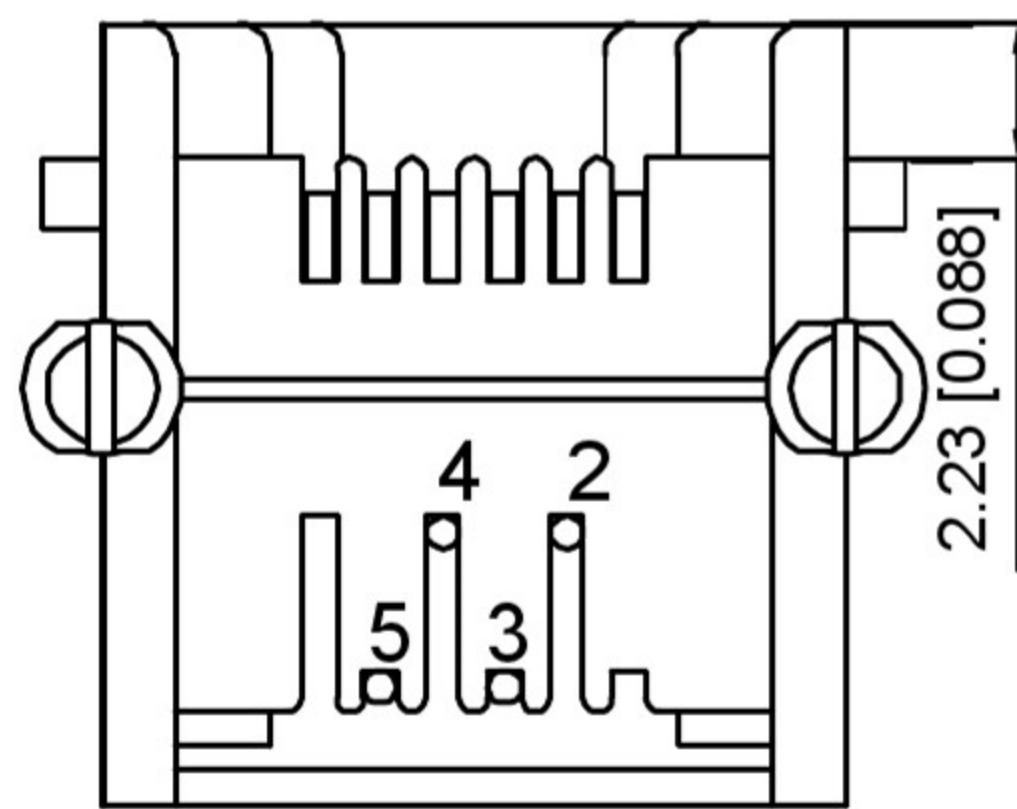
BOTTOM VIEW
