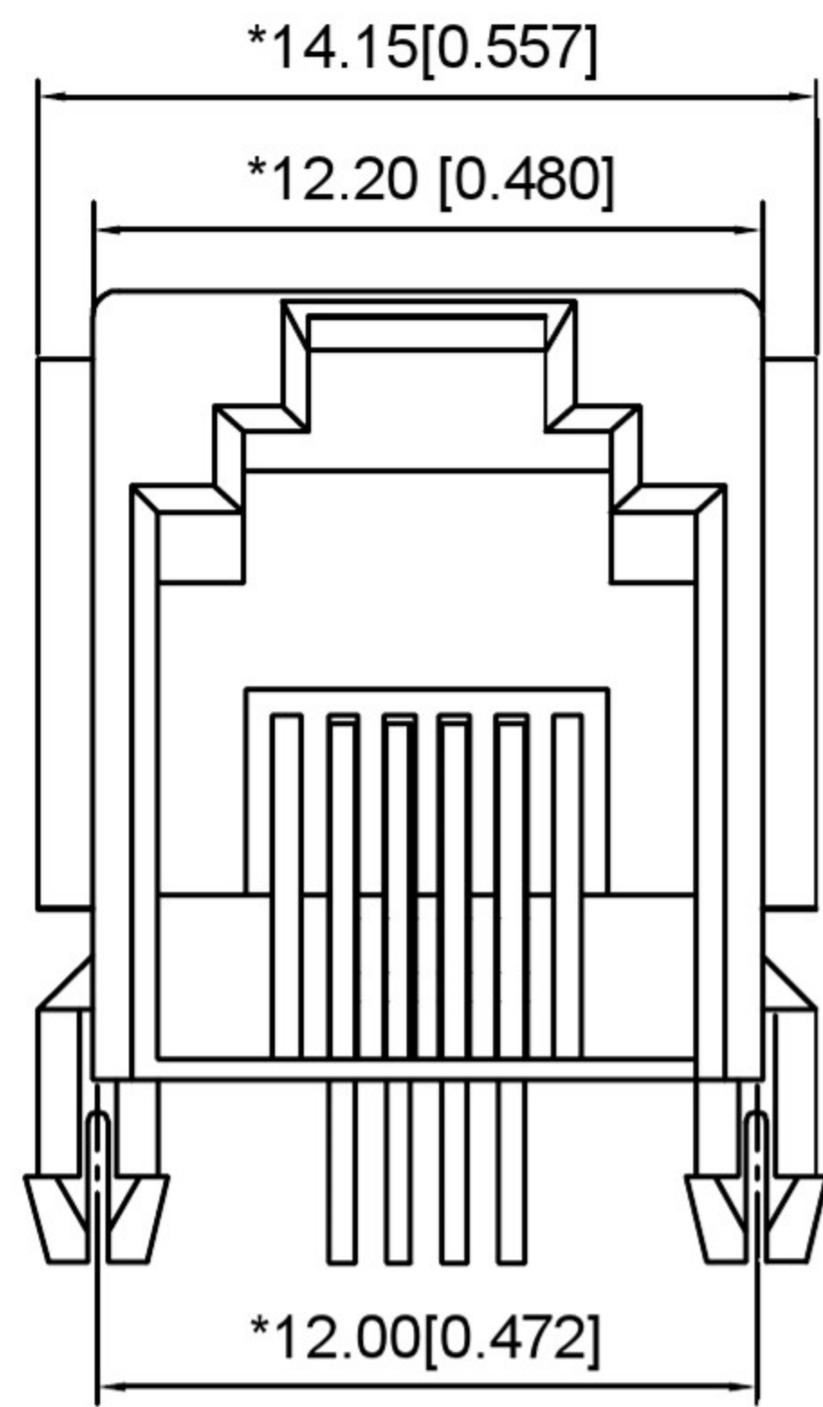
FRONT VIEW
