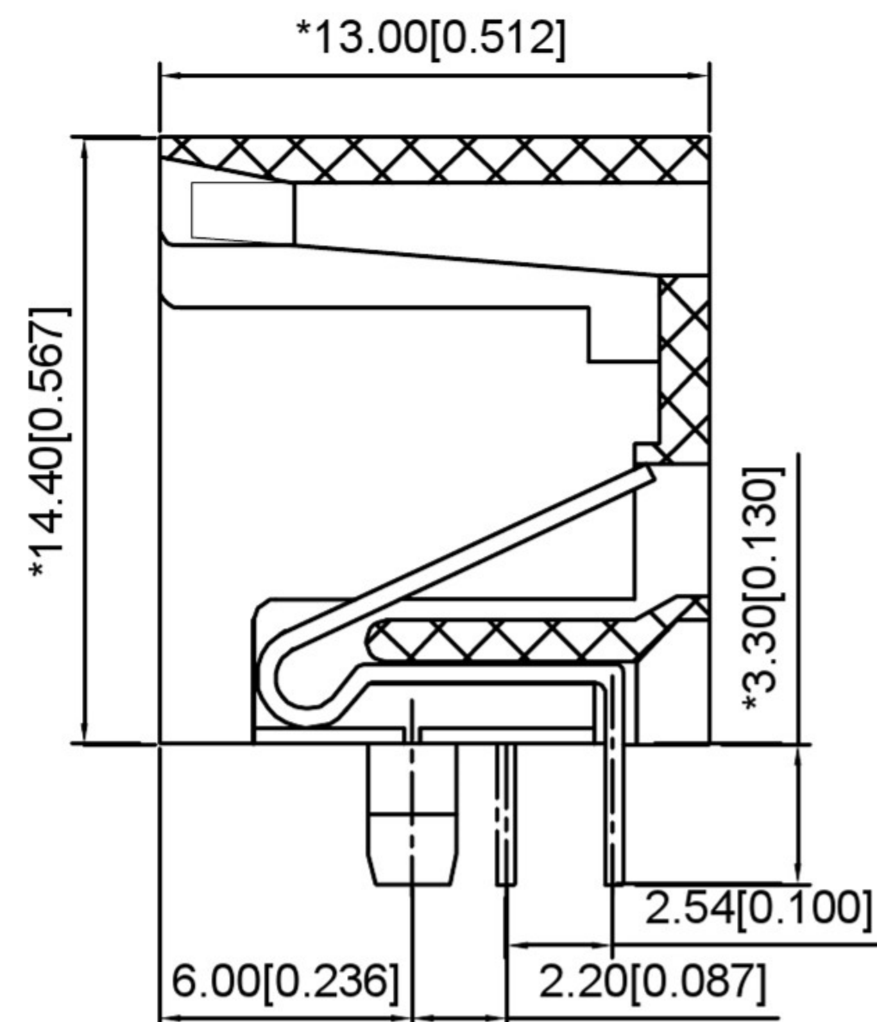
CUTAWAY VIEW
