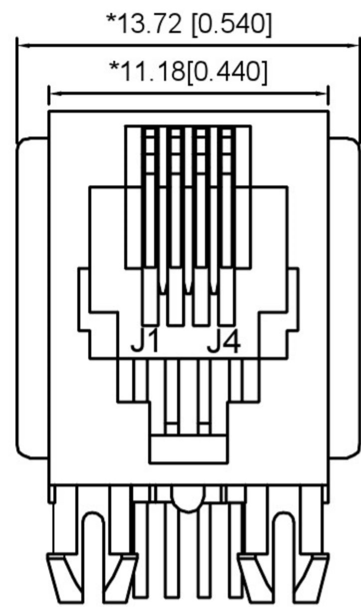
FRONT VIEW
