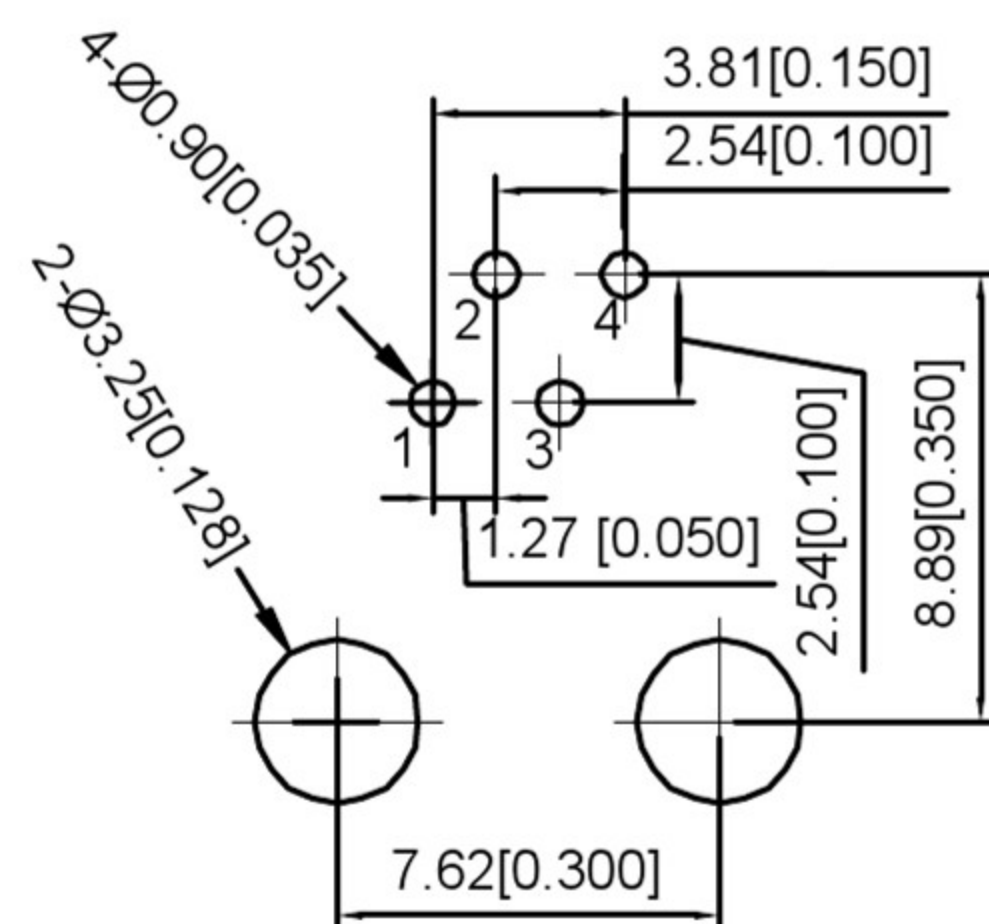
RECOMMENDED PCB LAYOUT VIEWED FROM COMPONENT SIDE
