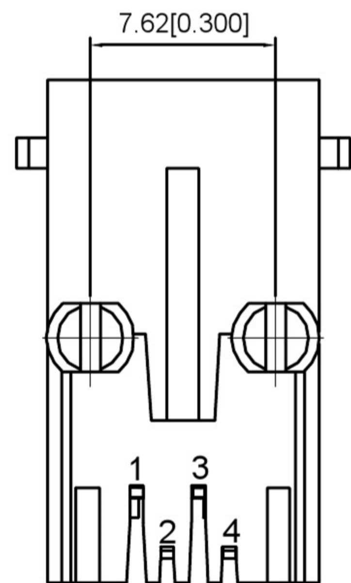
BOTTOM VIEW
