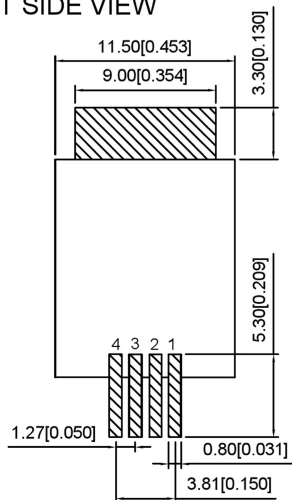
RECOMMENDED PCB LAYOUT VIEWED FROM COMPONENT SIDE
