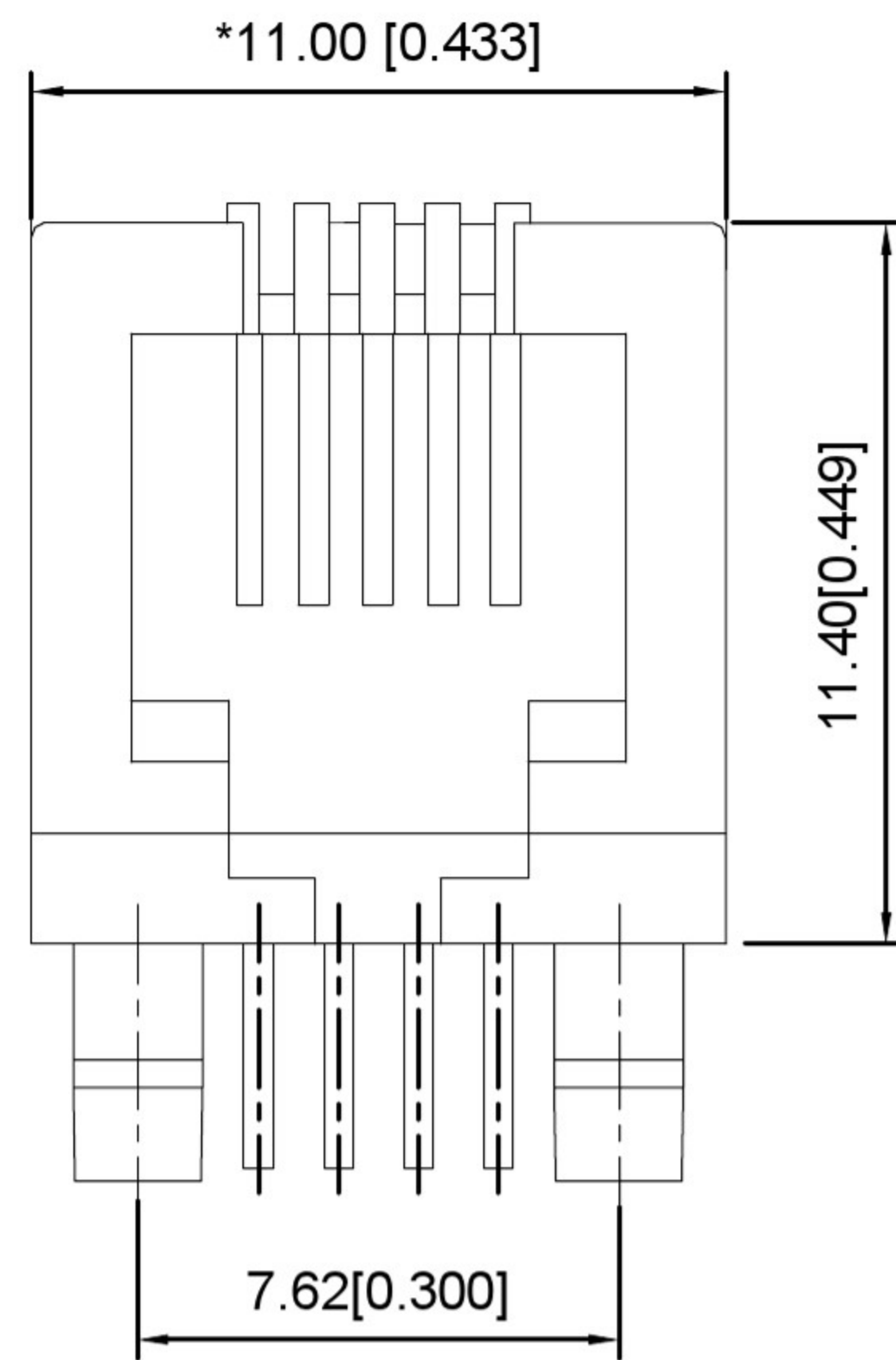
FRONT VIEW
