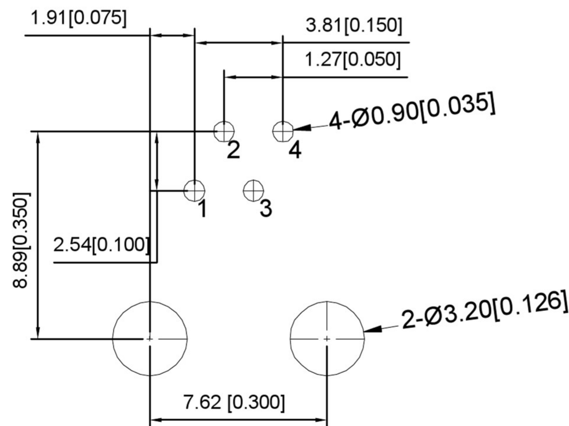
RECOMMENDED PCB LAYOUT VIEWED FROM COMPONENT SIDE
