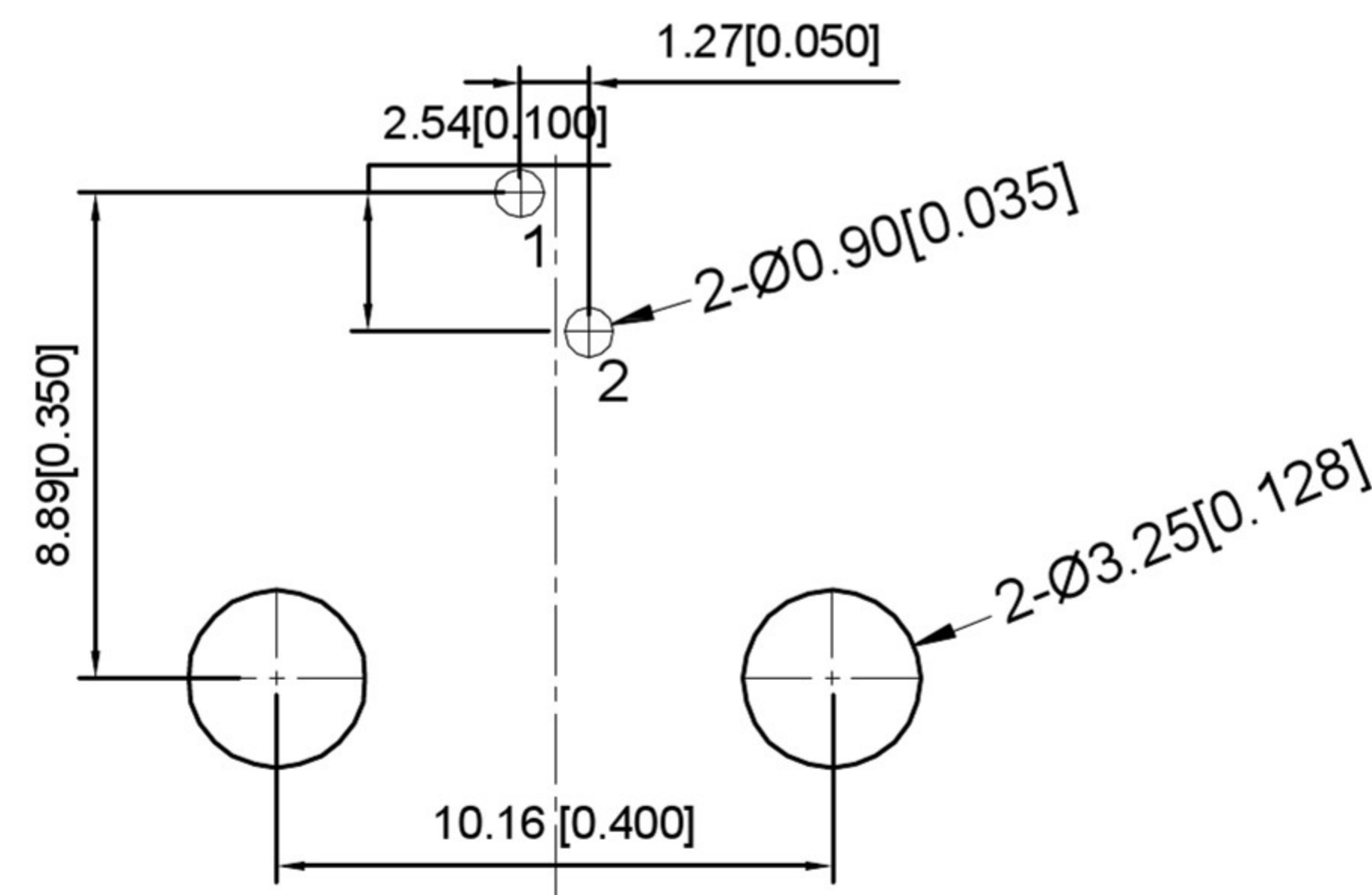
RECOMMENDED PCB LAYOUT VIEWED FROM COMPONENT SIDE
