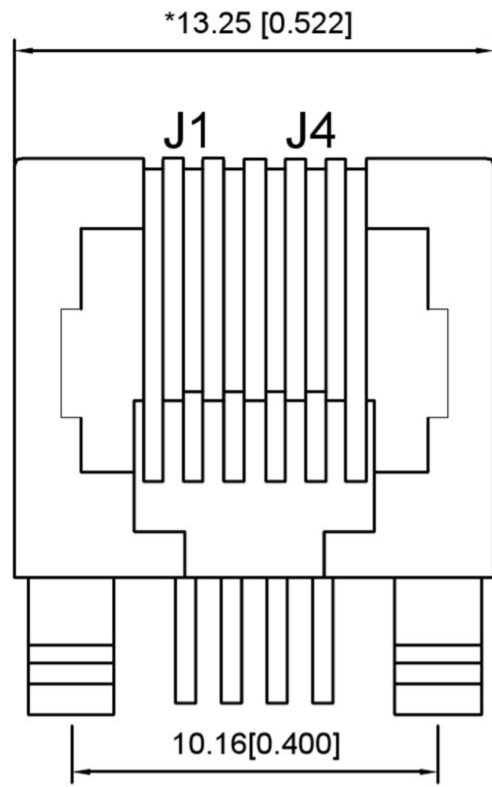
FRONT VIEW
