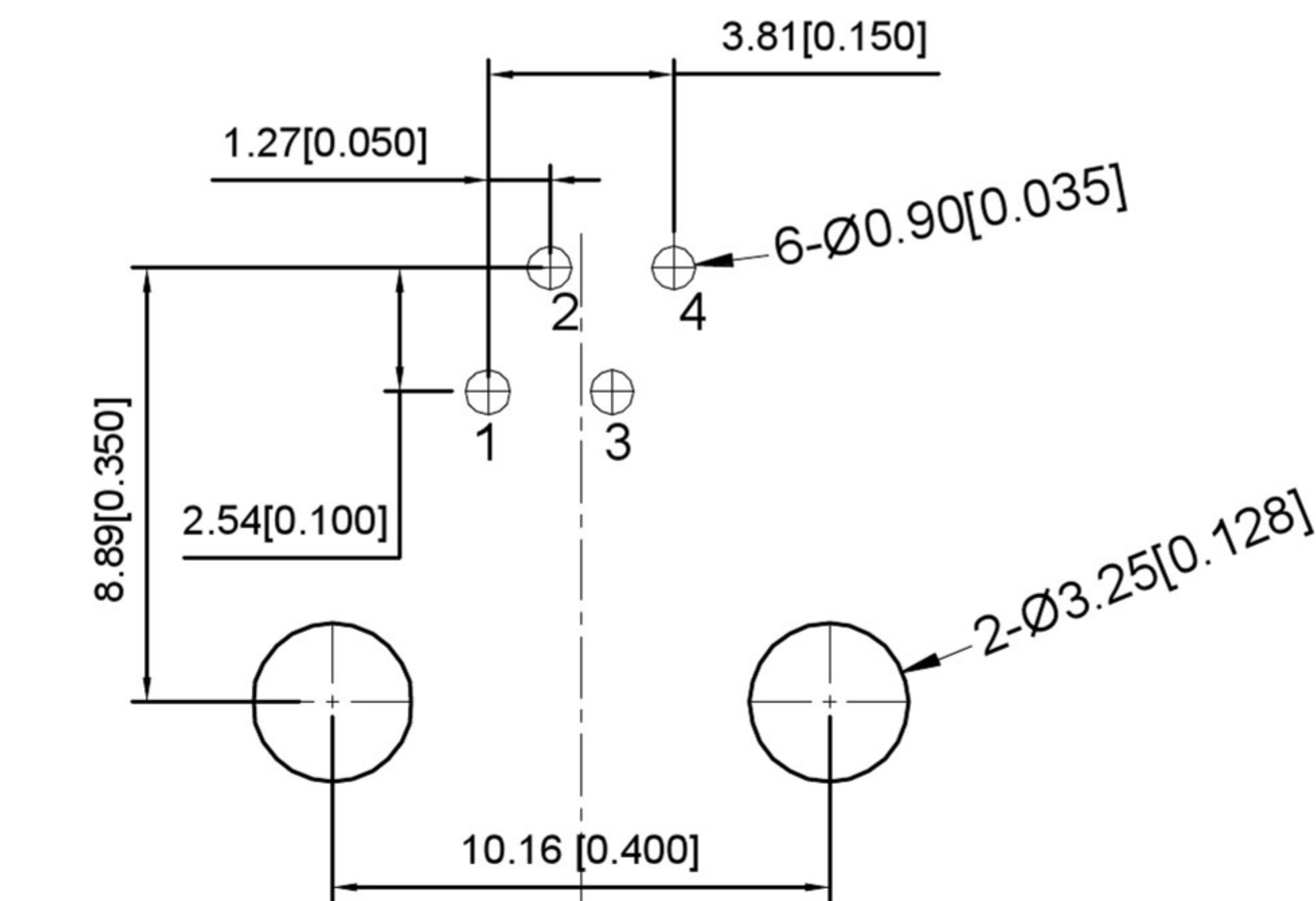
RECOMMENDED PCB LAYOUT VIEWED FROM COMPONENT SIDE
