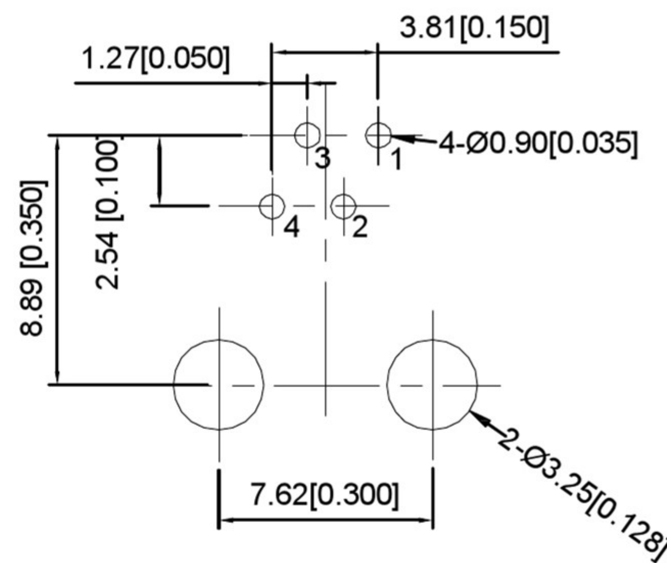
RECOMMENDED PCB LAYOUT VIEWED FROM COMPONENT SIDE
