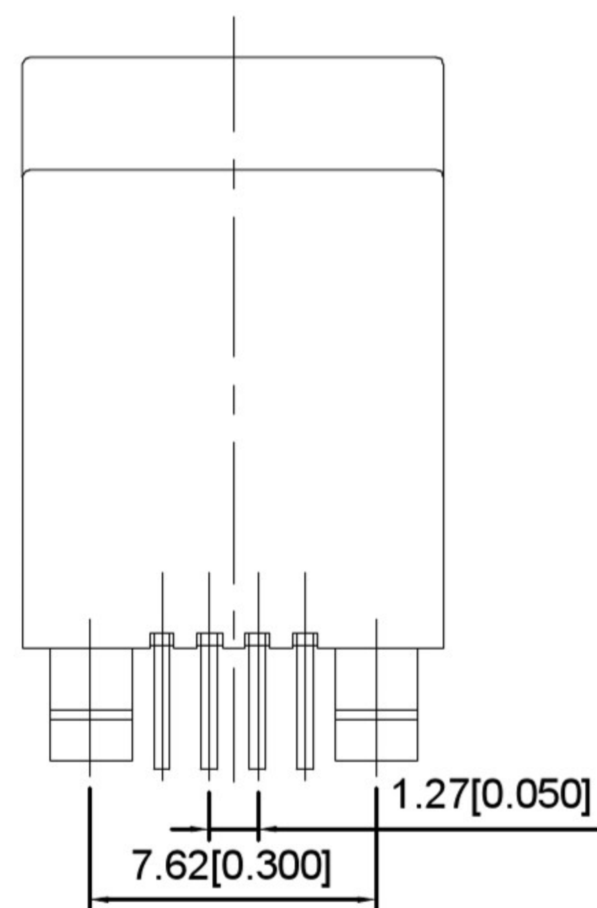
BOTTOM VIEW
