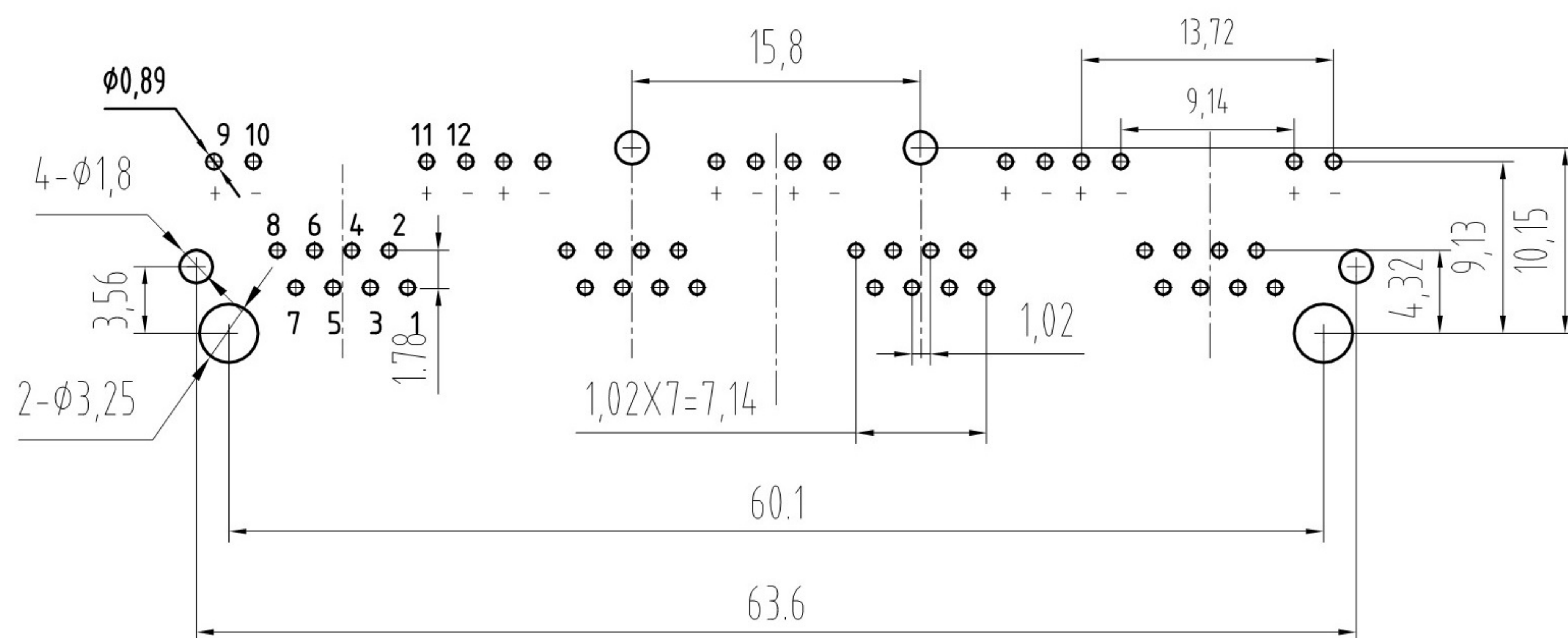
PC Board Layout Component Side Shown
