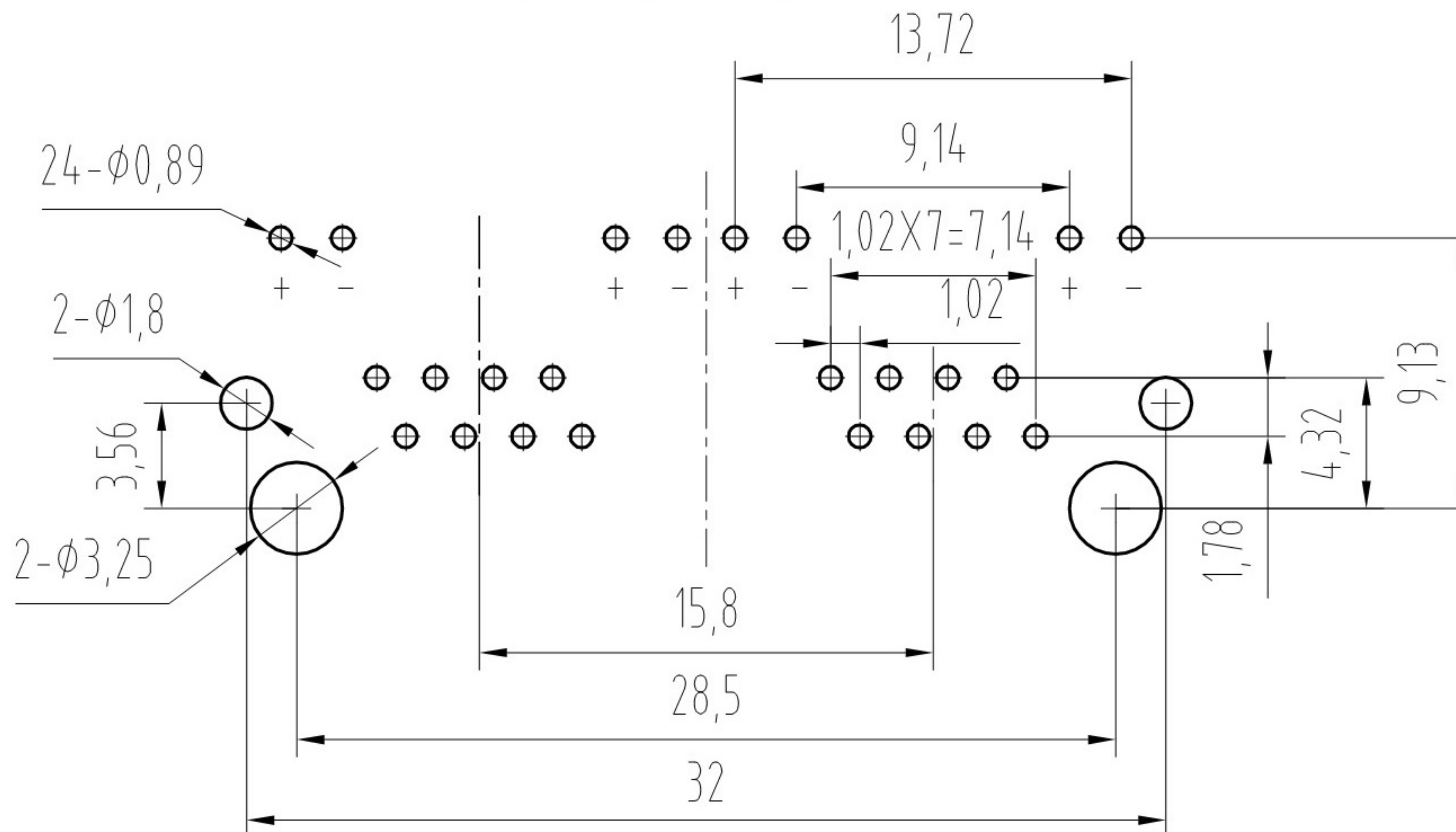
PC Board Layout Component Side Shown
