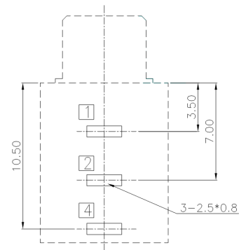
P.C.B LAYOUT(copper-sided view)
