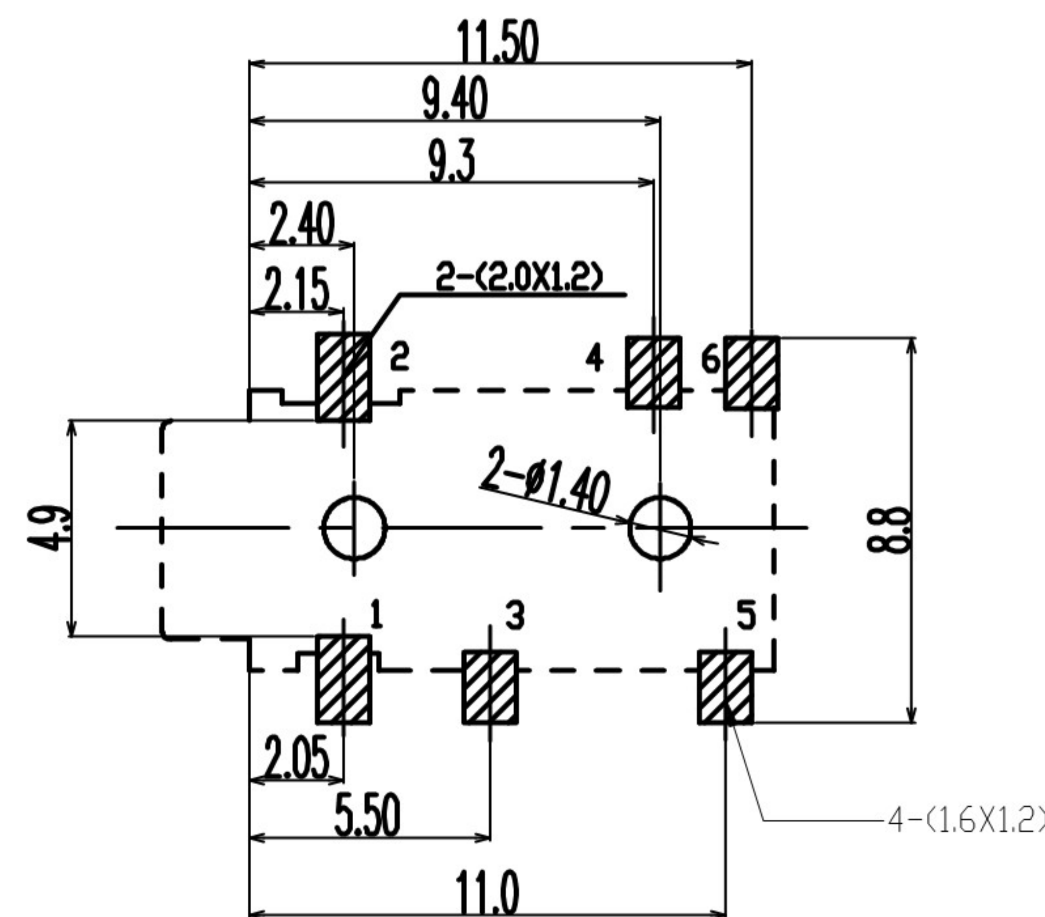
P.C.B LAYOUT TOP VIEW
