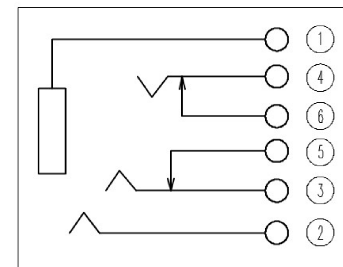
SCHEMATIC
