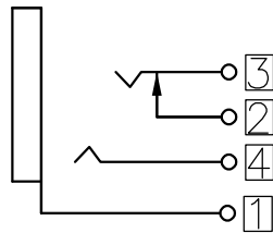
Electrical schematic
