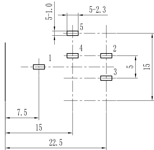
P. C. B LAYOUT (BOTTOM VIEW) Tolerance: ±0.05
