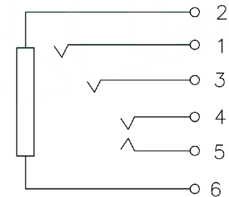
CIRCUIT DIAGRAM
