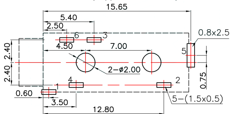
P.C.B LAYOUT(copper-sided view)
