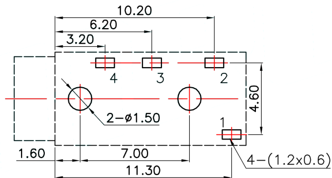
P.C.B LAYOUT(copper-sided view)
