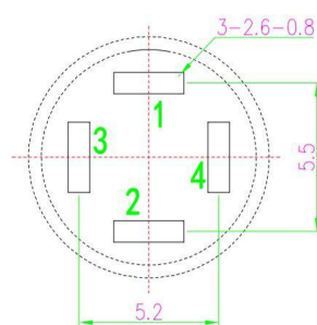
T:1.6 Dimensions of PC board holes Tolerance : \pm 0.1 (Printed-sided view)
