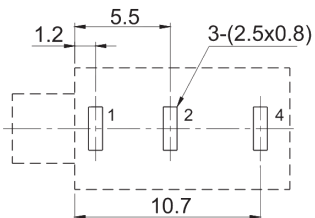
P.C.B Layout(copper-side view)
