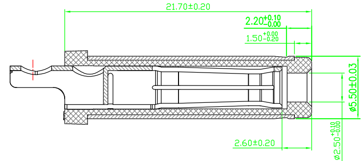
MATING PLUG DP550250-0188-60000H
